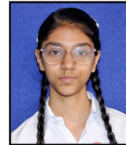
Mannat Overall 90.6%
